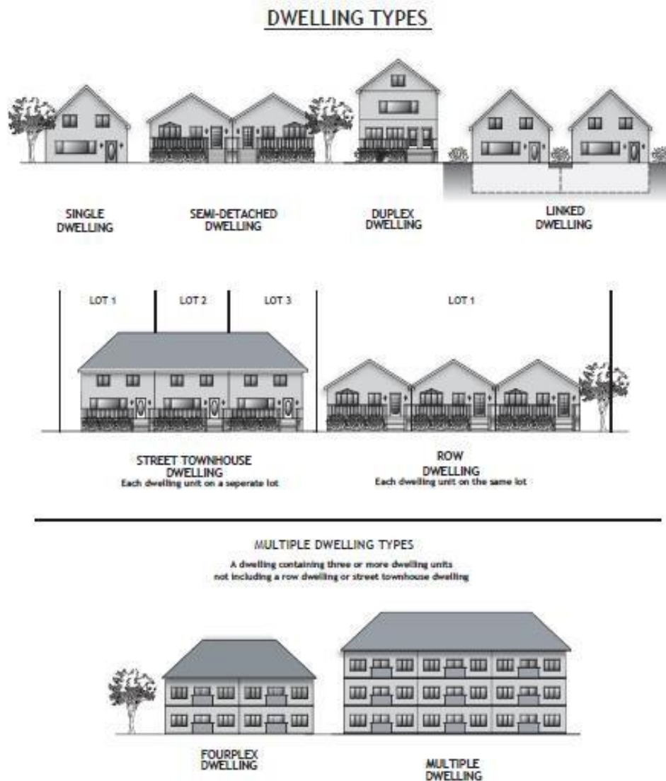
Figure 3.8: Dwelling Types
